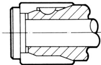
Standard half length
