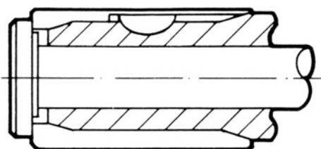
Extended length.
